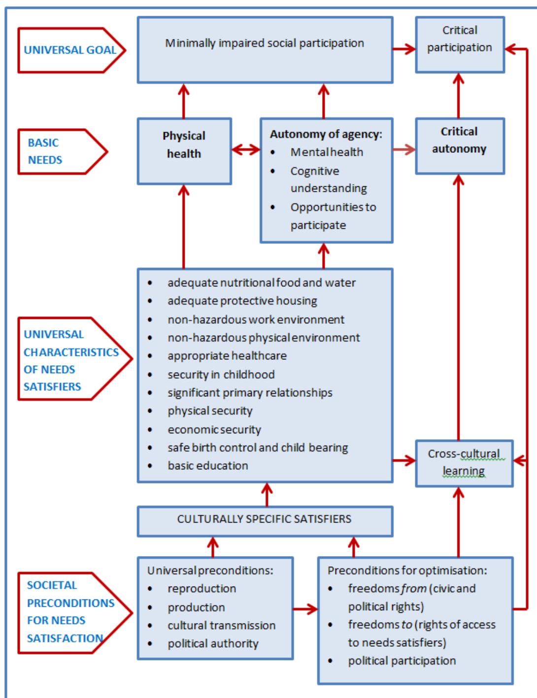
Figure 1. The theory of need in outline
